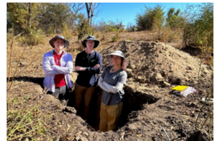
A hole dug for soil tests at bridge site in Zambia (June 2024)
